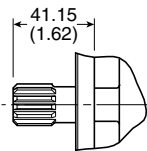
SHAFT OPTION "B" (SAE "B") 13 TEETH 16/32 PITCH 30° INVOLUTE SPLINE MAX. TORQUE = 208.1 N·m (1,850 IN-LBS)
